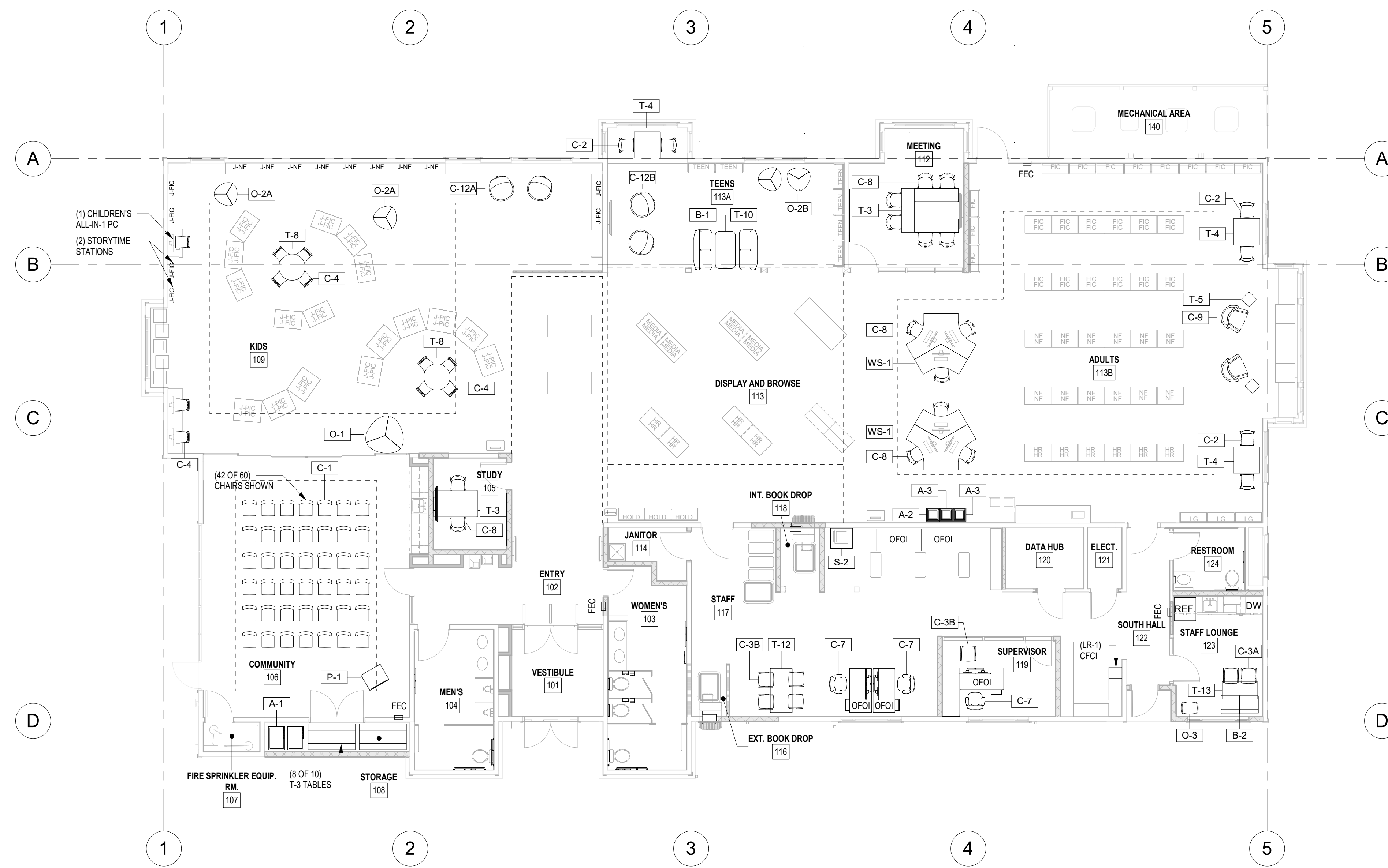
1 FURNITURE PLAN A115 1/8" = 1'-0"
